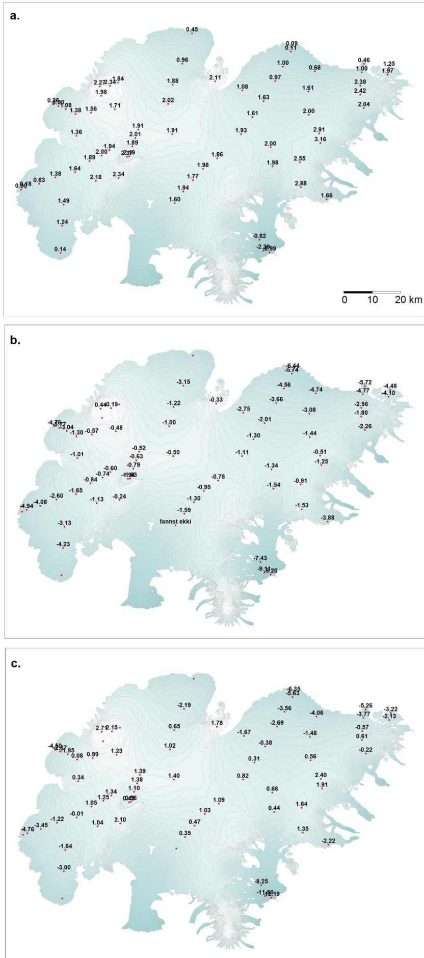
Figure 2. Maps showing point values of specific surface mass balance in m_{we} , 2022_23. a. winter, b. summer, c. net balance.
