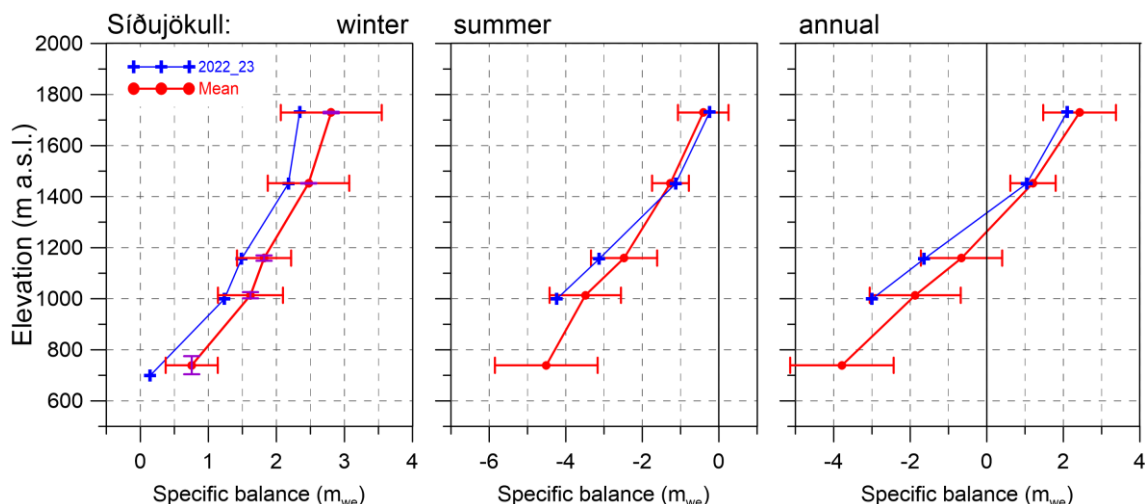
Figure 13. Mass balance at a central flow line of Síðujökull 2022_23 and average mass balance 2004_05 to 2021_22.
