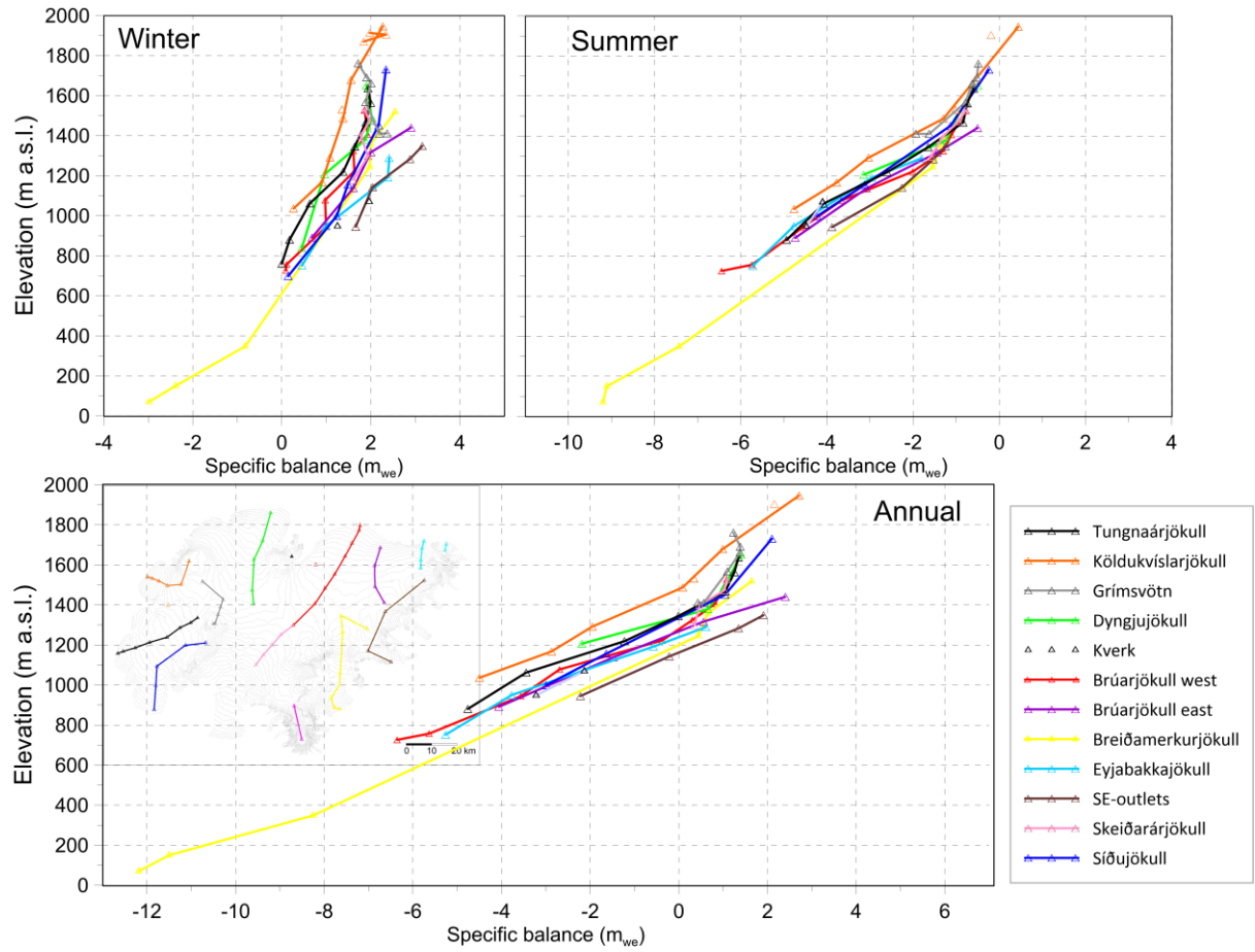
Figure 3. a. Specific mass balance ( m_{we} ), at survey sites along all mass balance profiles 2022_23.
