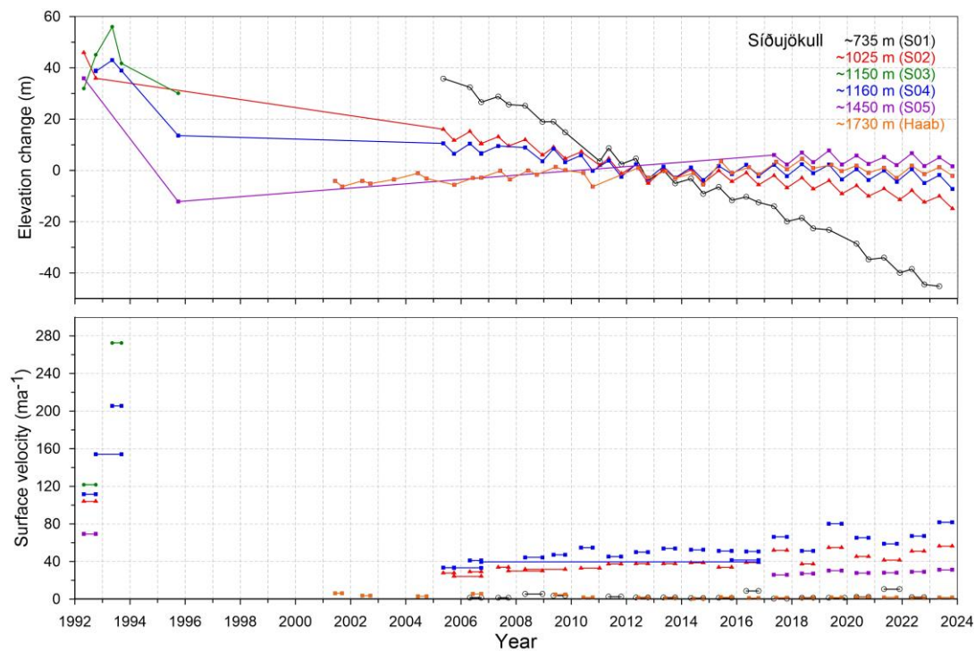
Surface elevation change relative to summer 2012 (upper panel) and average surface velocity at mb sites (lower panel) on Sídújökull in 1992 to 2023.
